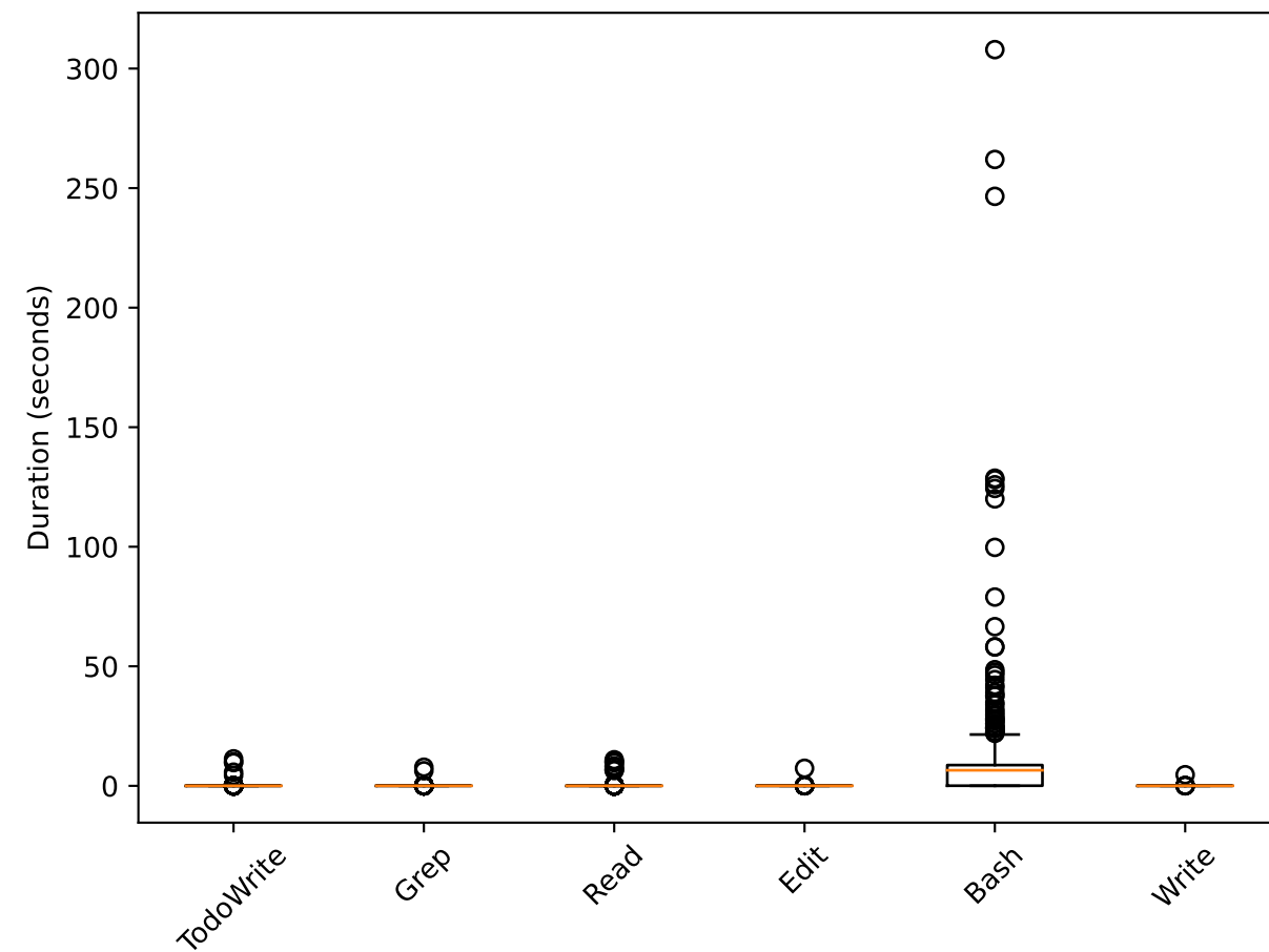
Tool Execution Time Distribution
