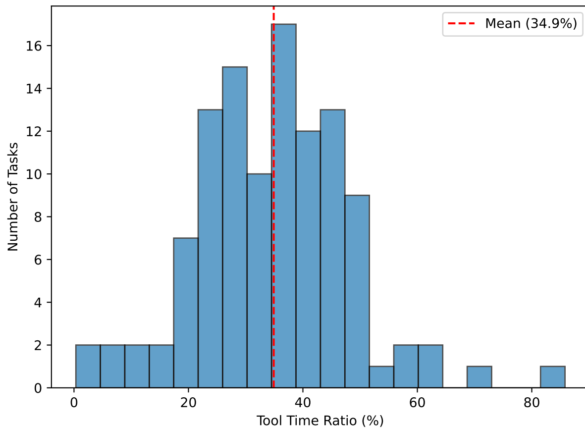
Distribution of Tool Time Ratios
